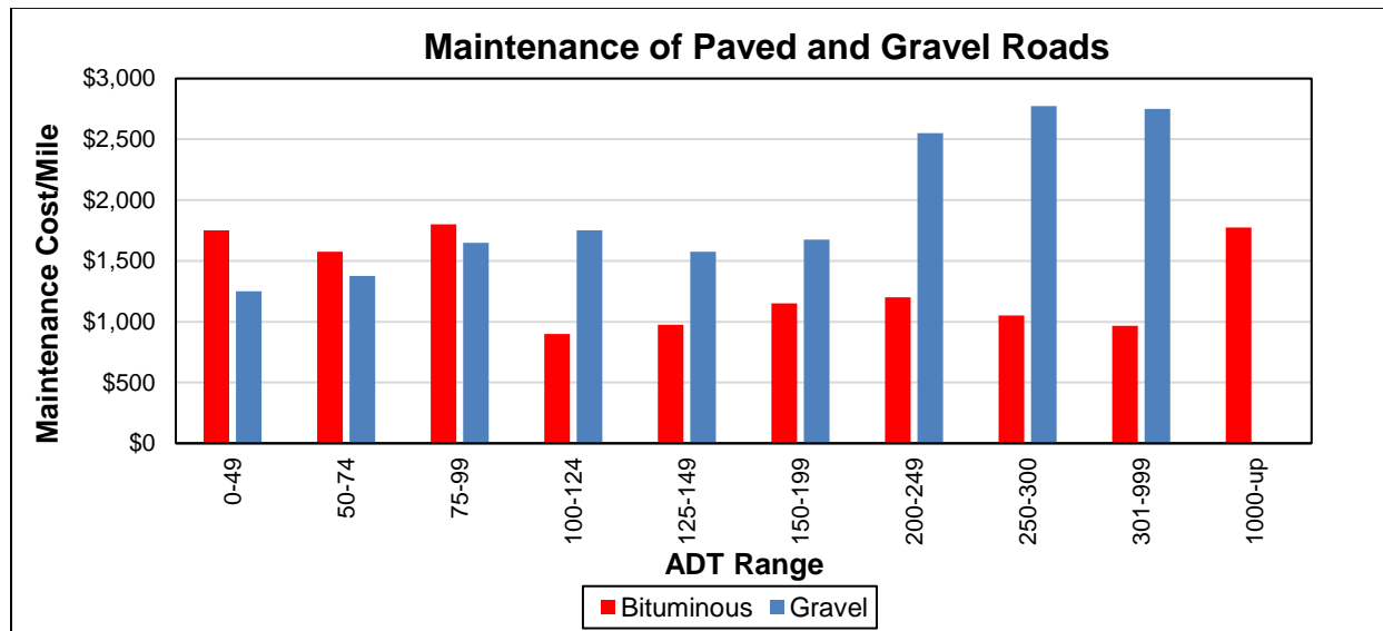
Figure 14: Economics of Upgrading an Aggregate Road (The Minnesota Local Road Research Board, 2005)
