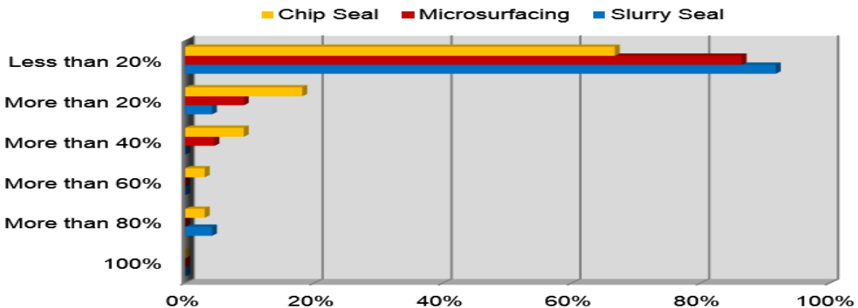
Figure 4: Application of Preventive Treatments According to Best Practices
